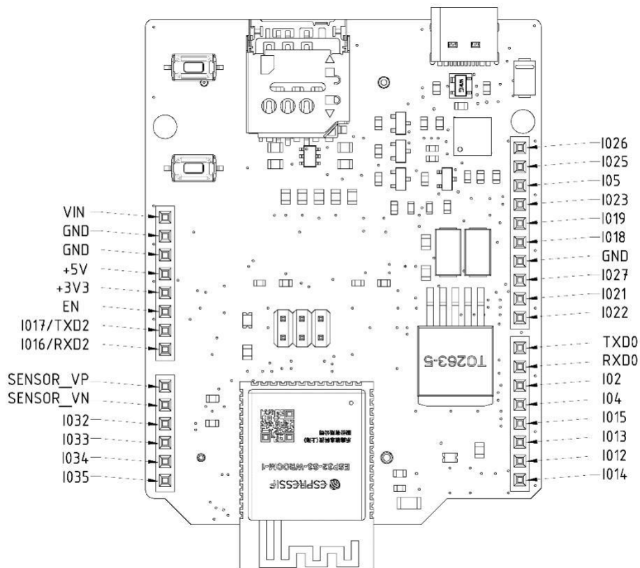
Figür 1: Cellron Pin Layout
